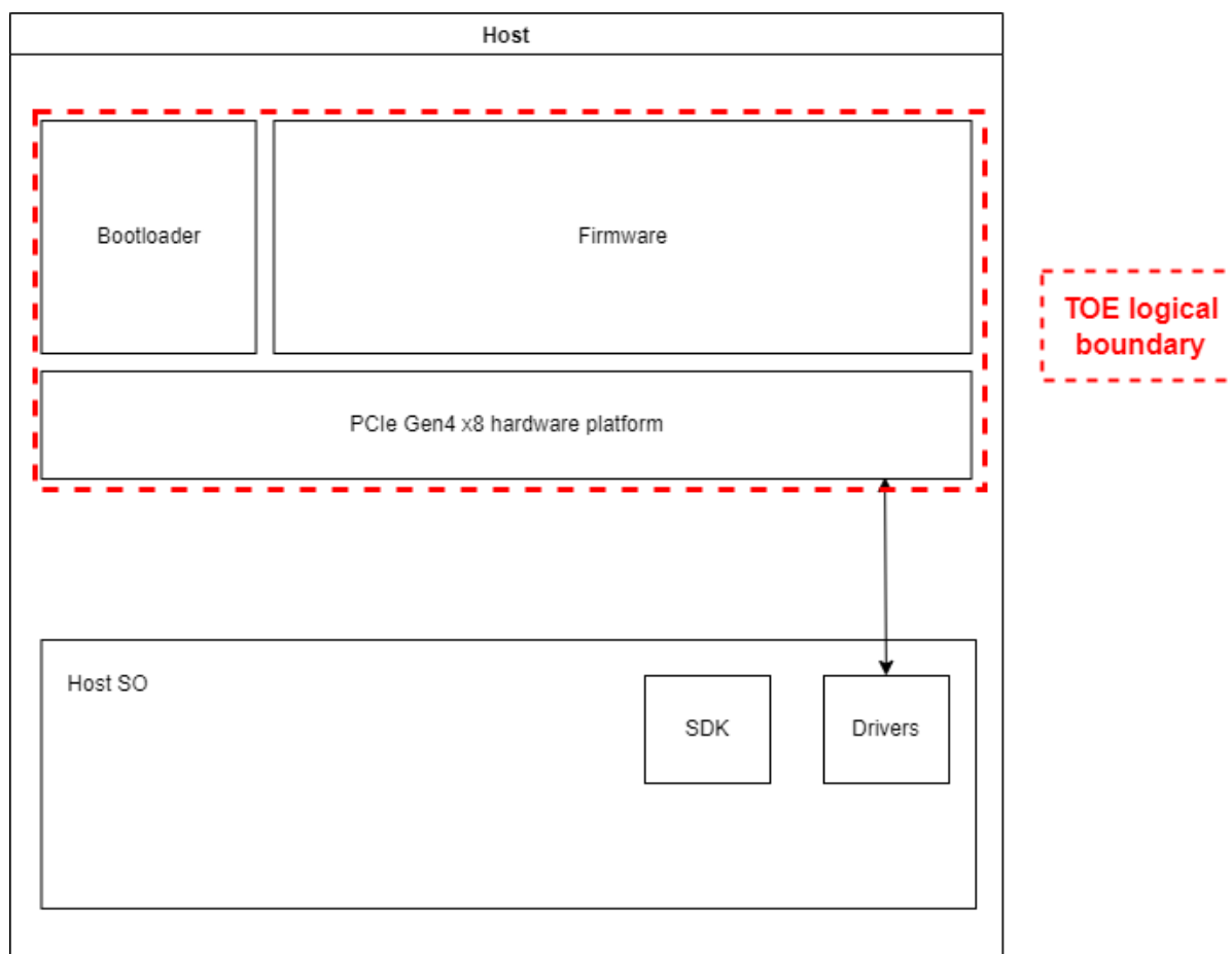
Figure 2 TOE logical boundary
