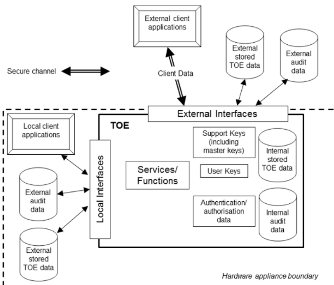
Figure 1 Generic TOE Architecture
